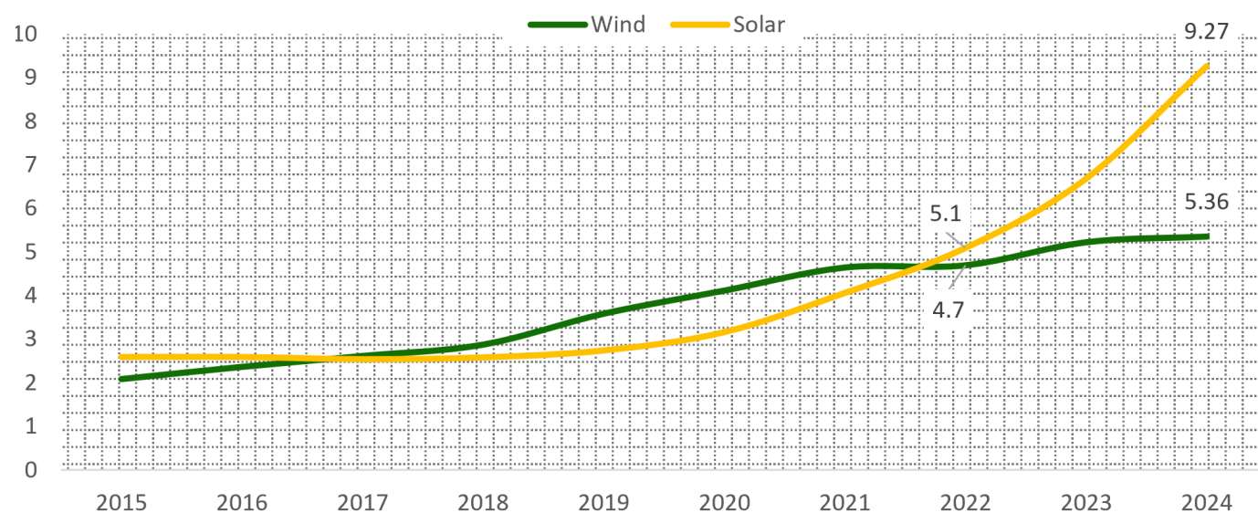
Figure 8. Solar & Wind Evolution in Greece bottom (GW), [2015 - 2024]. Source: Ember
